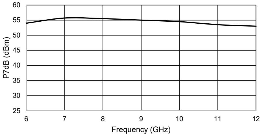
P7dB vs Frequency
