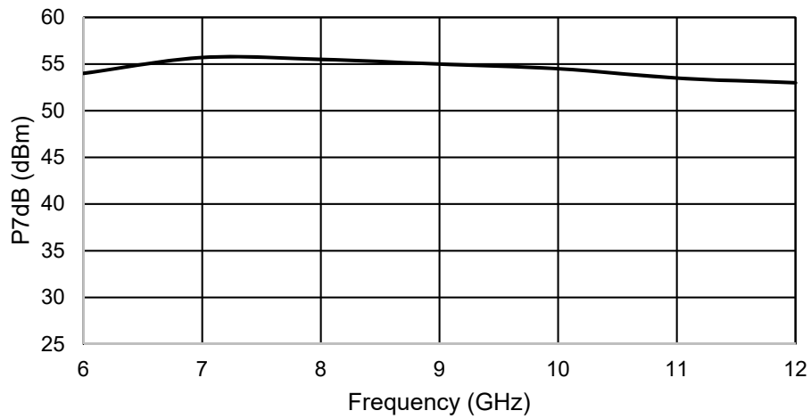
P7dB vs Frequency
