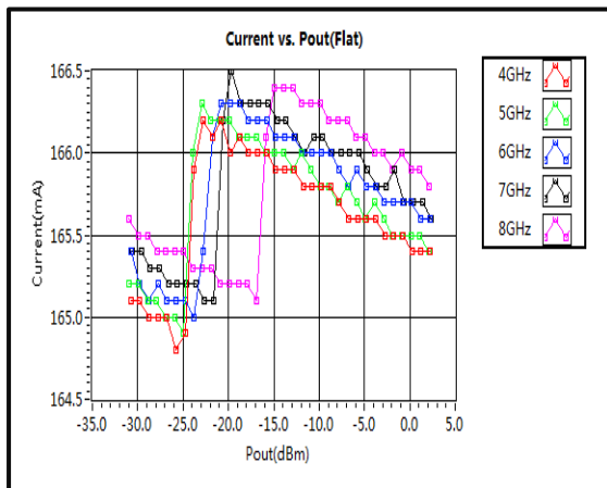
Current vs. Pout(Flat)
