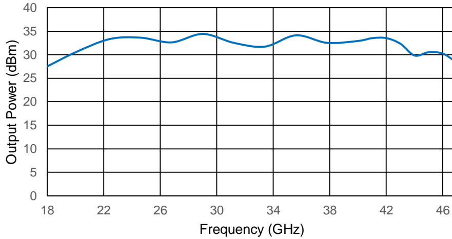
P1dB vs Frequency
