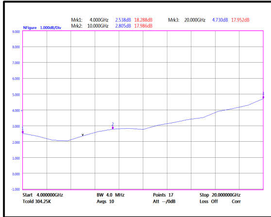
Noise Figure(4GHz-20GHz)
