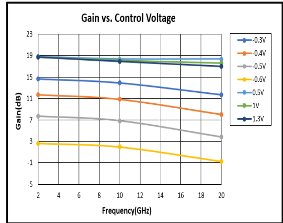
Gain vs. Control Voltage
