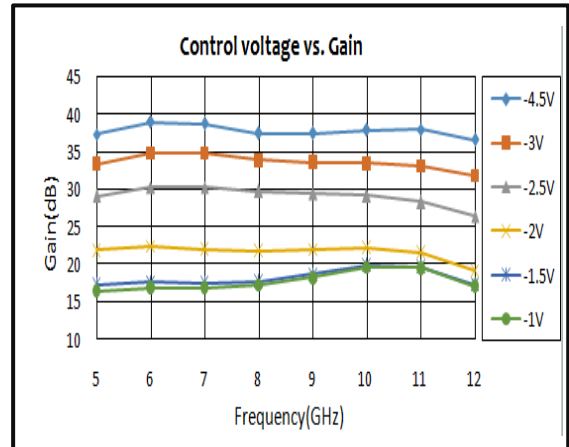
Control Voltage vs. Gain
