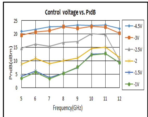
Control Voltage vs. P1dB
