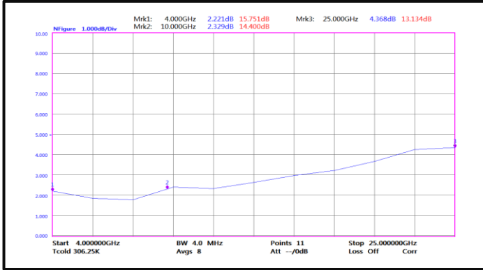
Noise Figure (4GHz-25GHz)
