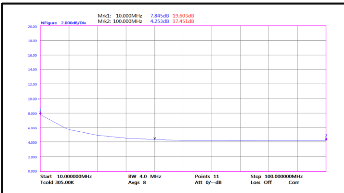
Noise Figure (10MHz-100MHz)
