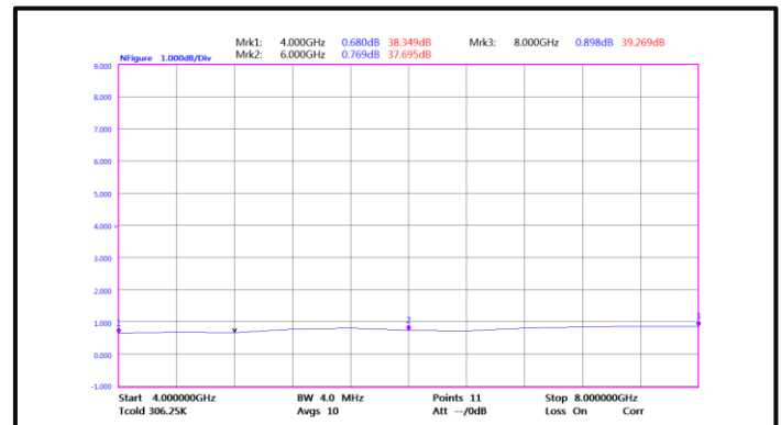
Noise Figure(4-8GHz)
